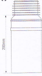
Straight Extension. 3 1/2"/90mm Outlet.
