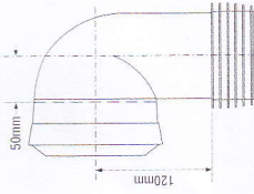
90° Bend. 4"/110mm Outlet. Non Adjustable.
