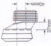
40mm Offset. 4"/110mm Outlet.
